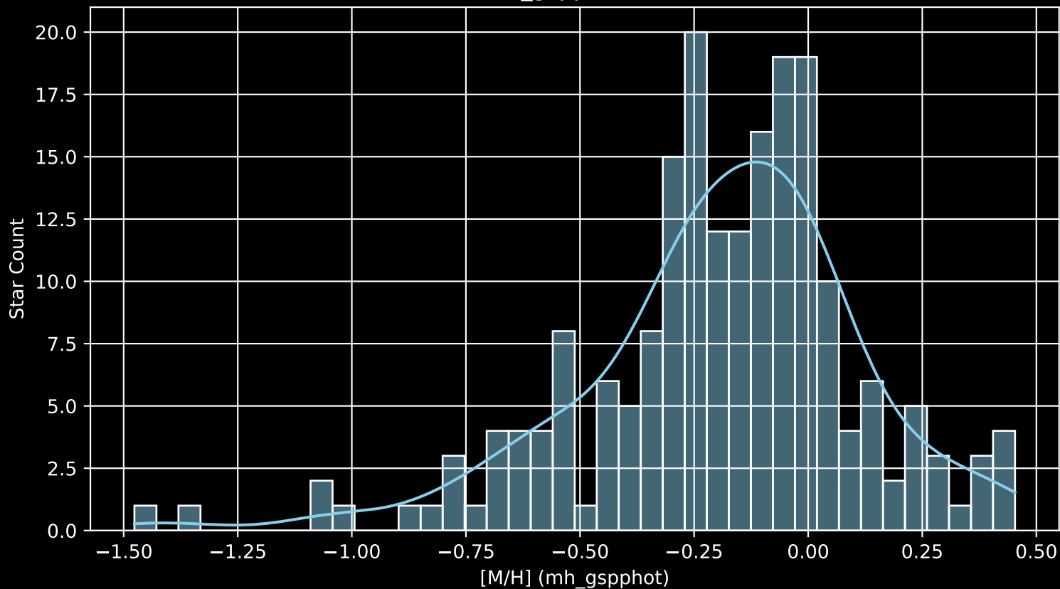
APOGEE DR17 Field: [084-40_MGA [M/H] (mh_gspphot) (n= 202)
