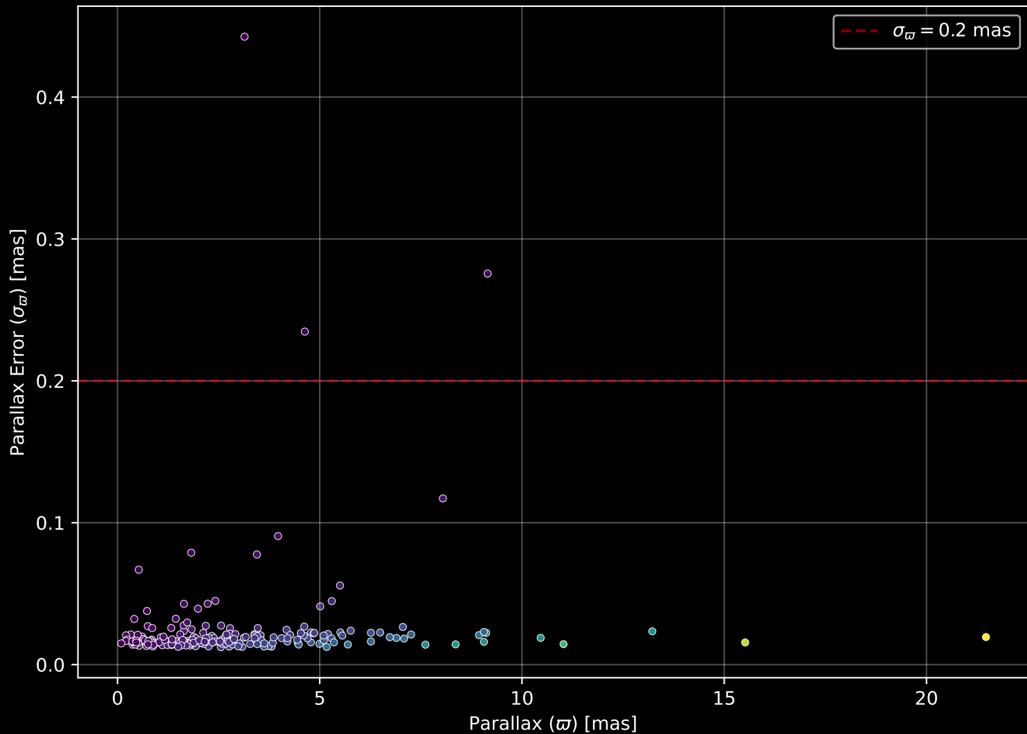
APOGEE DR17 Field: [084-40_MGA] Parallax Quality (n= 206)
