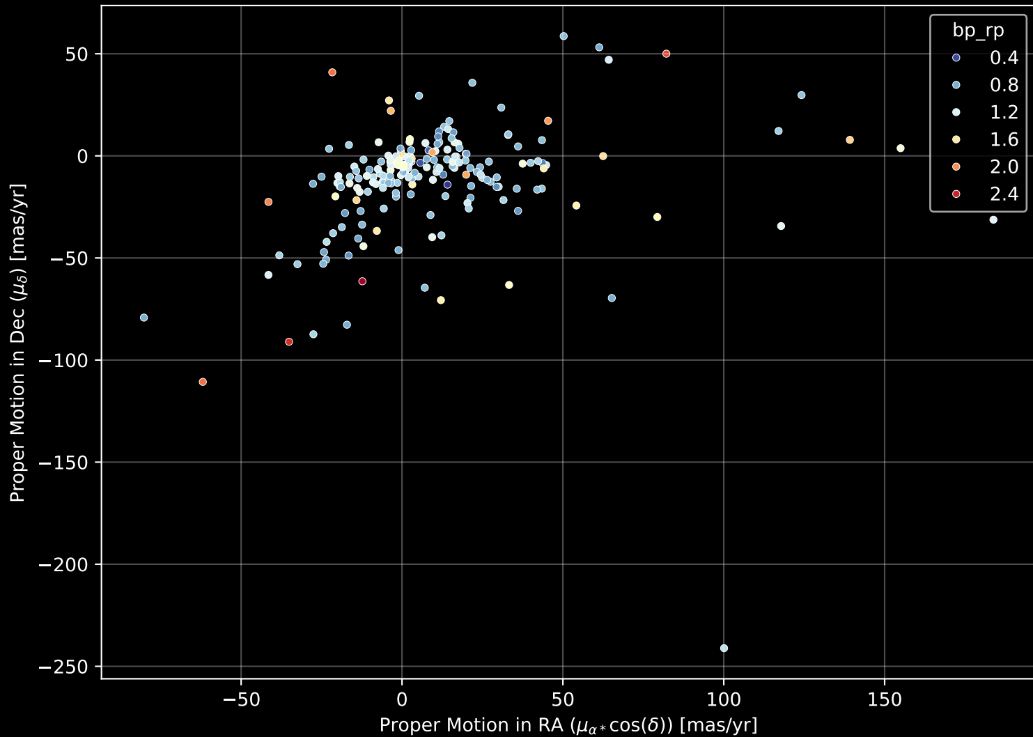
APOGEE DR17 Field: [084-40_MGA] Proper Motion Diagram (n= 206)
