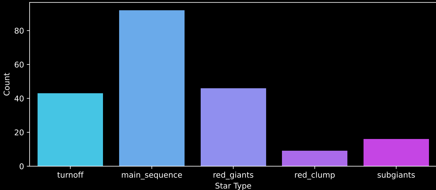
APOGEE DR17 Field: [084-40_MGA] Count plot of Star Type
