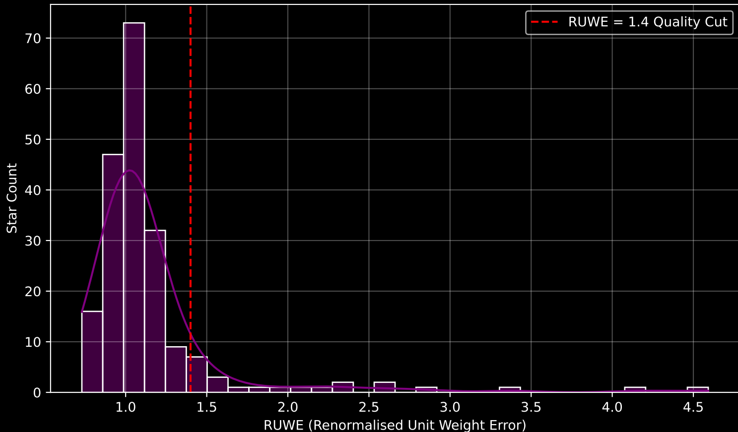
GAPOGEE DR17 Field [084-40_MGA] RUWE Distribution (n= 200)
