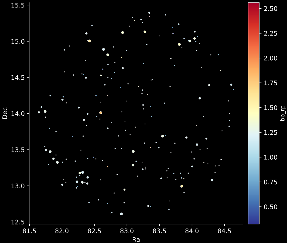
APOGEE DR17 Field: [084-40_MGA] Stars: 206
